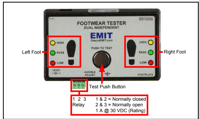
Figure 3. Dual Independent Footwear Tester features and components
